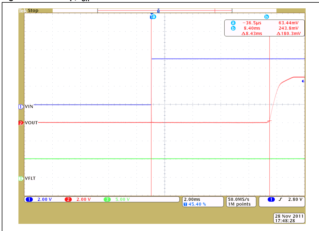
Figure 10. Startup, t_{on}
